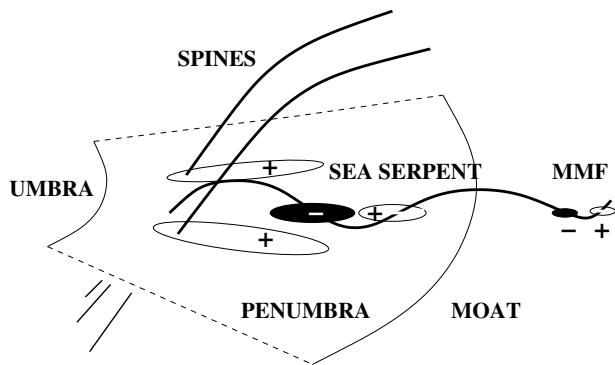
Fig. 3. Sketch of the penumbra showing sea-serpent field lines between more vertical spine fields. The ovals indicate the polarity of the different structures when observed at disk center.
