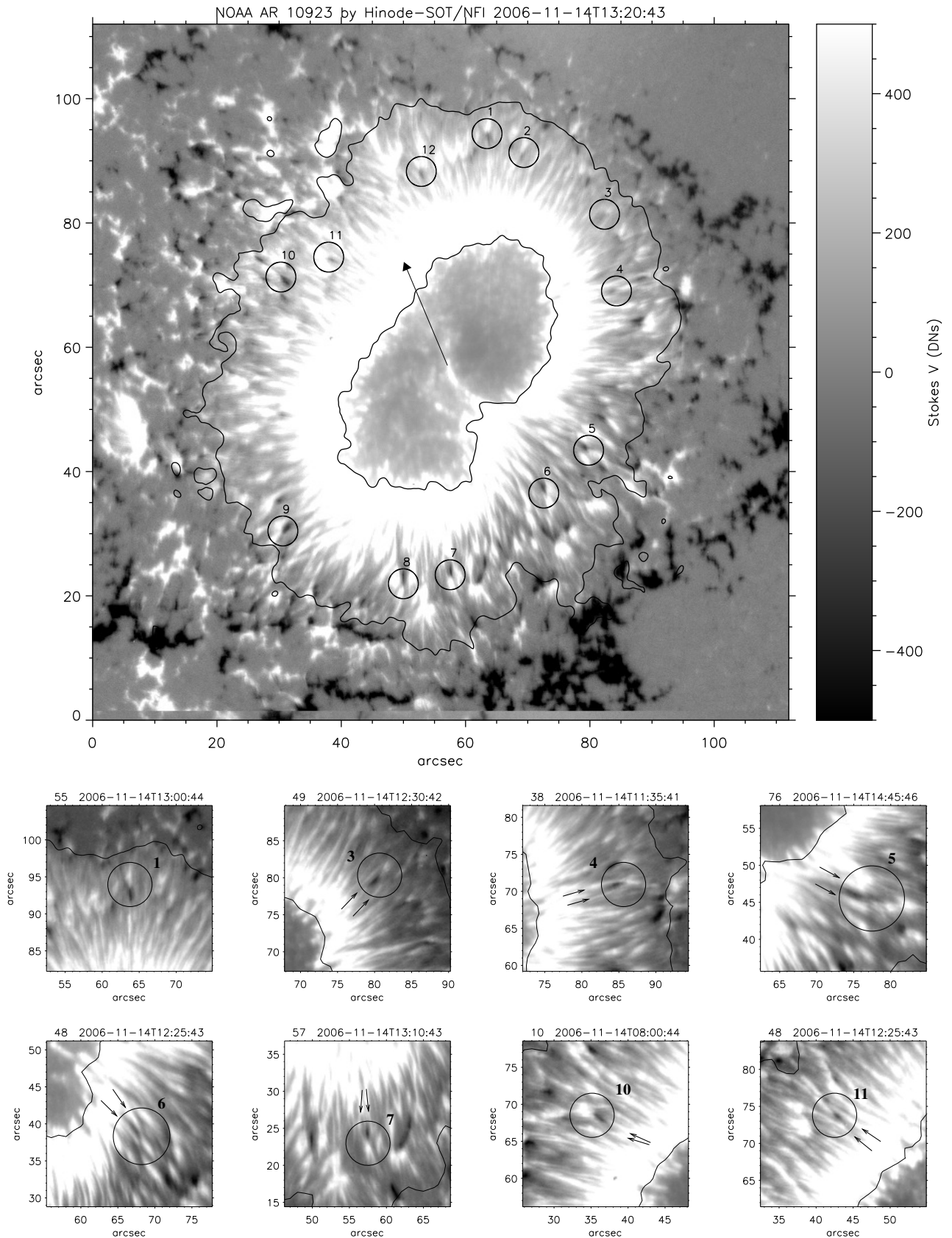
Fig. 1. Top: Magnetogram (Stokes V map) of AR 10923 with umbral and penumbral contours overlaid. The magnetogram signal has been reversed to treat the spot as if it were of positive polarity. The direction to disk center is marked with an arrow. The circles indicate a number of negative-polarity signals in the penumbra. The magnetogram is saturated at \pm 500 data numbers (hereafter DN). Bottom: 22''.5 \times 22''.5 subfields showing some of the negative-polarity patches. Usually, they are associated with a positive-polarity structure farther from the umbra. The bipolar pairs occur in between filaments of positive polarity (indicated with arrows). The frame number and time of each magnetogram is given in the title.
