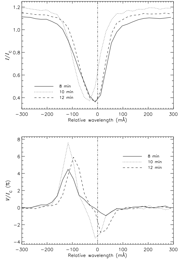
Fig. 3. Stokes I (top) and V (bottom) profiles of Fe I 630.25 nm from the center of the magnetic flux concentration studied in Fig. 1. The solid, dotted and dashed lines correspond to \Delta t = 8, 10 , and 12 minutes, respectively. The vertical line mark the zero point of the velocity scale.
